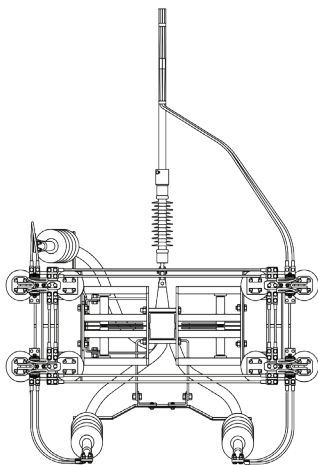
Installation of the disconnector and four motor drives on one pole.
